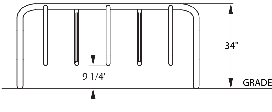
ELEVATION VIEW
